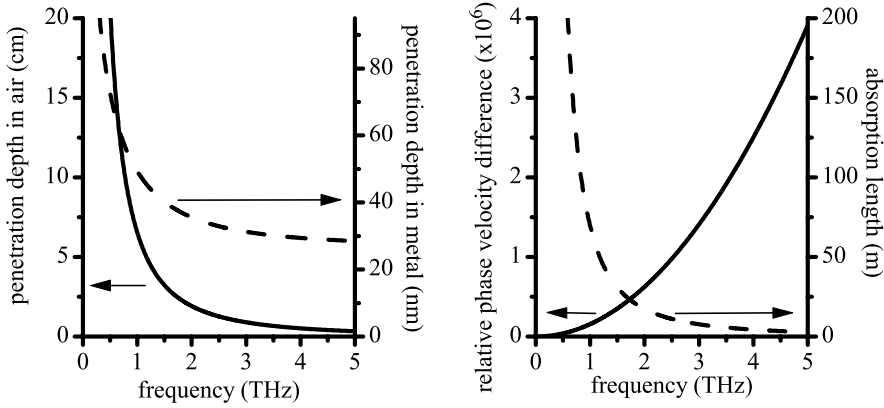
Figure 5.3: Calculated frequency dependence of the properties of a plasmon-polariton propagating on a planar copper-vacuum interface. The left graph shows the penetration depth both in air and in copper. The right graph displays on the left axis the difference between the plasmon-polariton phase velocity and the vacuum velocity of light divided by the vacuum velocity of light. The right graph also shows the absorption length of the plasmon-polariton (right axis).
