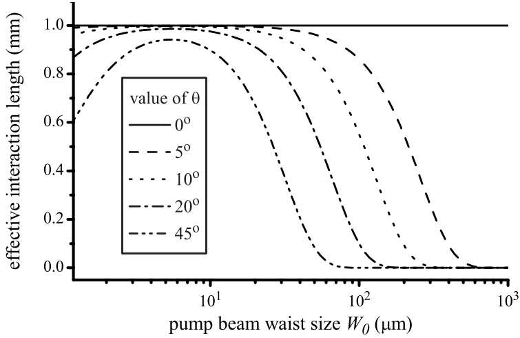
Figure 4.4: Calculated effective generation length ( AB ) as a function of the pump beam waist size W_0 . The values that are used are z_2 = 0.5 mm, z_1 = -0.5 mm, k_T = 2\pi \cdot 3 / (150 \mu\text{m}) , and k(\omega) = 2\pi \cdot 3 / (1 \mu\text{m}) .
