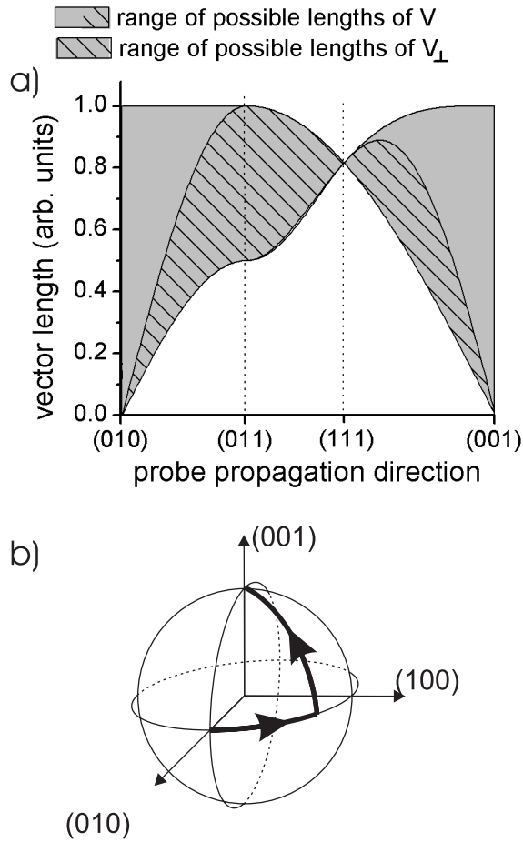
Figure 2.3: a) Values that can be obtained for the length of \mathbf{V} and the length of the component of \mathbf{V} perpendicular to \hat{\mathbf{s}} ( \mathbf{V}_\perp ) as a function of the probe propagation direction. b) The path followed for the propagation direction displayed on the horizontal axis of graph a.
