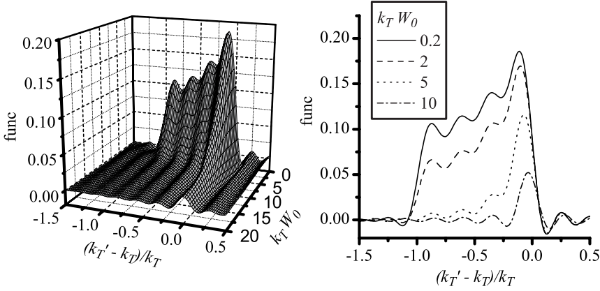
Figure 4.6: Graphs of \text{func}(k_T W_0, 50, (k'_T - k_T)/k_T) , which plays an important role in equation 4.40 for the focussed radiated field. The right graph shows cross-sections of the 3D graph on the left for different values of k_T W_0 .
