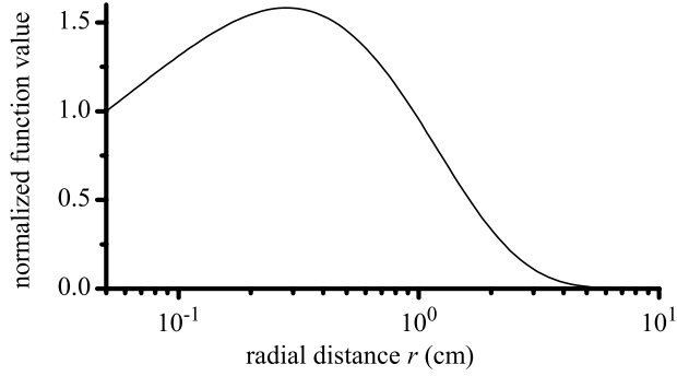
Figure 5.8: The radial dependence of the r|H_0^{(1)}(\kappa_a r)|^2 function, which is relevant to estimate the influence of a neighbouring object, for a plasmon polariton propagating over a 1 mm thick copper wire at a frequency of 0.54 THz. The function is normalized to 1 at the surface of the wire.
