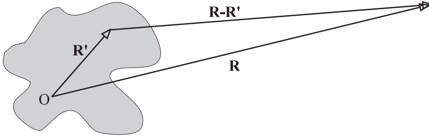
Figure 4.3: Geometry used to calculate the radiation produced by a limited area (grey) with an arbitrary distribution of currents and charges. O indicates the origin, \mathbf{R}' the generation point and \mathbf{R} the observation point.
